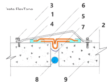
Fig: Typical Drawing & Detailing of Expansion Joint Sealing System with Da 'Crete FlexTape
